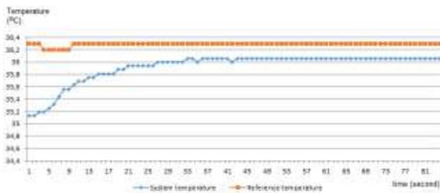
Figure 14. Result of the fifth experiment for temperature testing process
